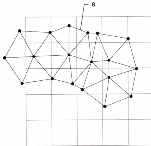
Figure 1: Voronoi Polygons
